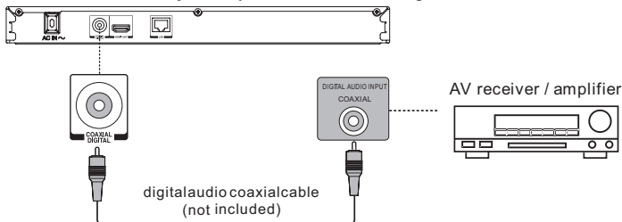
(Sample Illustration) Connecting to a digital amplifier/AV receiver
