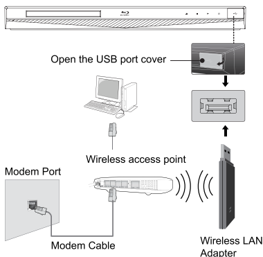
(Sample Illustration) Connecting to a wireless router
