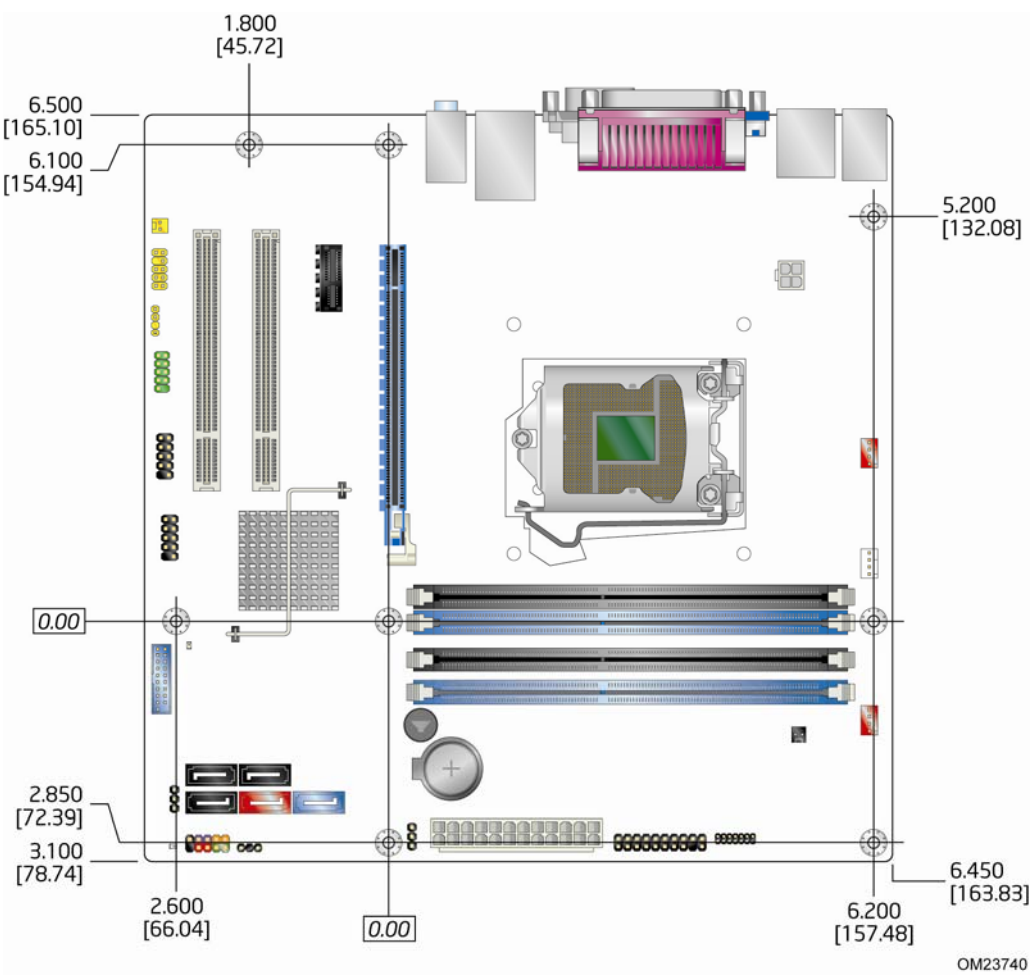
Figure 16. Board Dimensions
