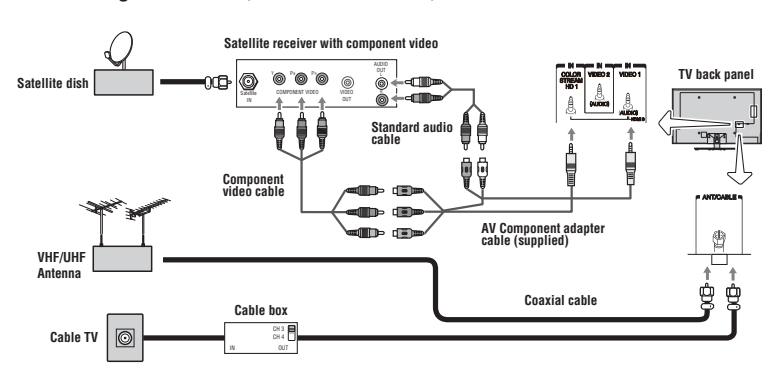
(Sample Illustration) Connecting to an antenna, satellite receiver, and cable TV box.
