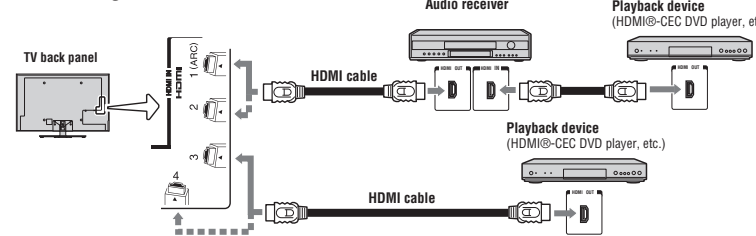
(Sample Illustration) HDMI®-CEC connections
