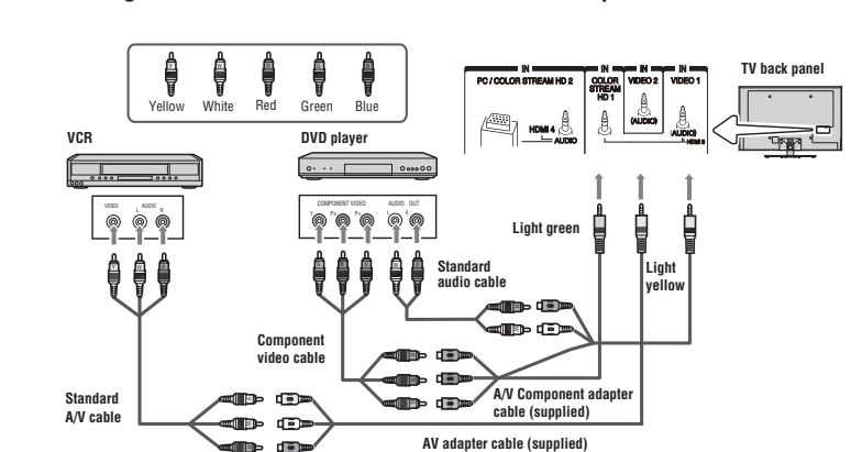
(Sample Illustration) Connecting a DVD with ColorStream® or a VCR with composite video
